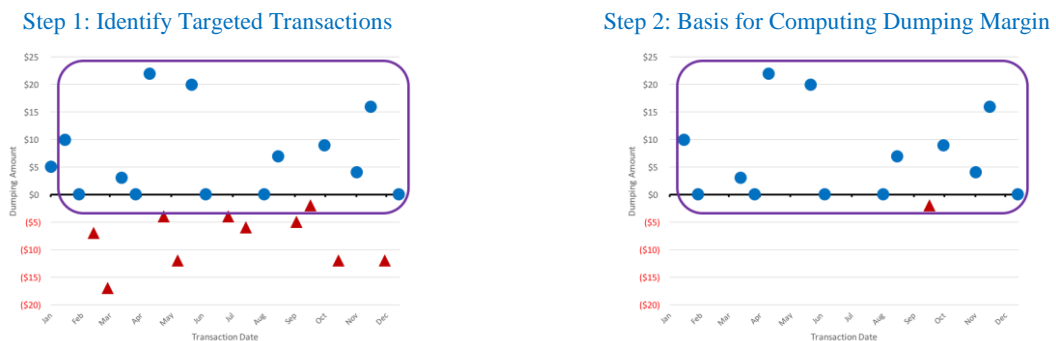
Figure 7: Backdoor Zeroing
