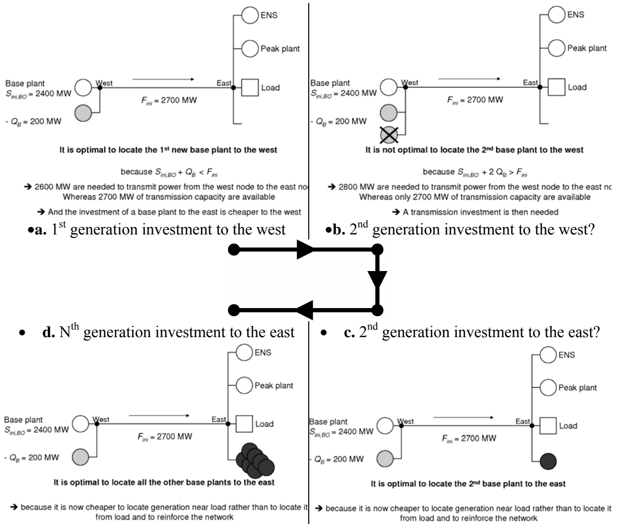
Fig. 8. Optimal sequence of generation investments when the initial transmission capacity is 2700 MW
