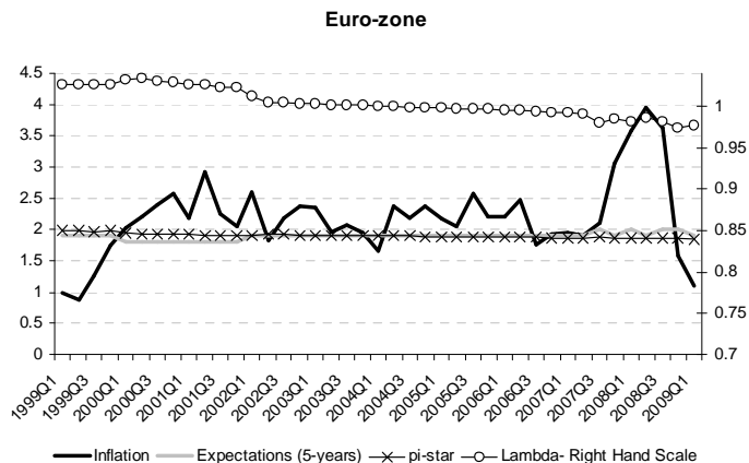
Figure 5: Time-varying \lambda .
