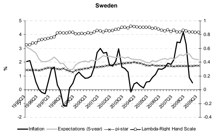
Figure 3: Time-varying \lambda .
