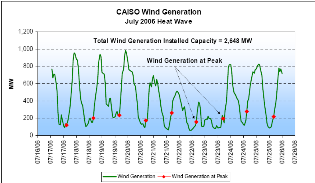
Figure 3 California Wind Generation During 2006 Heat Wave
