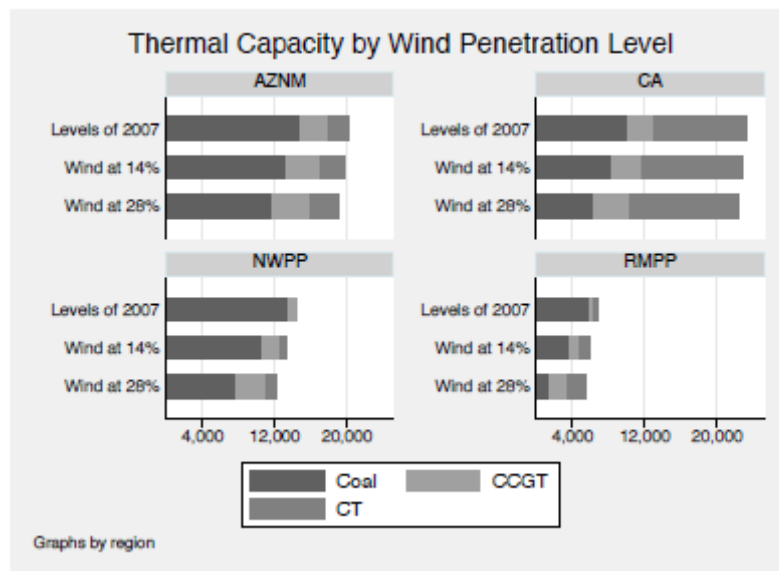
Figure 10. Equilibrium capacity investment with $25/ton CO 2
