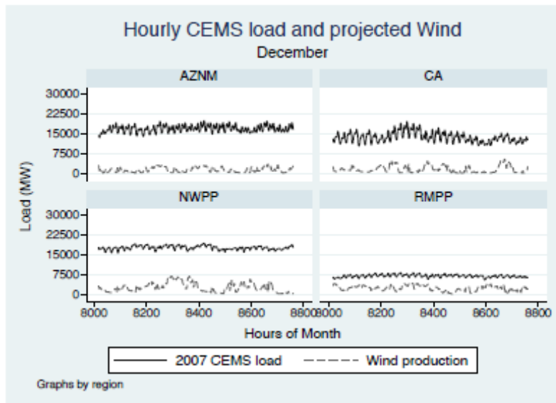
Figure 3. CEMS load and wind production for December
