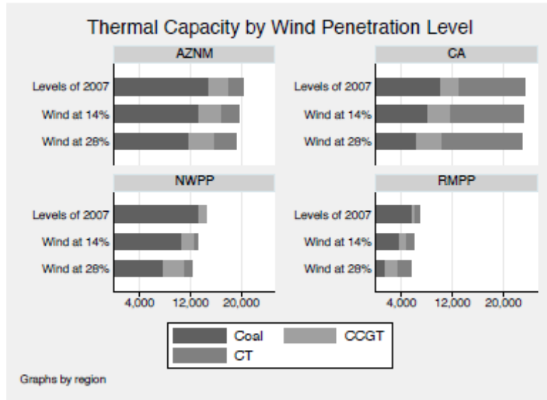
Figure 7. Equilibrium capacity for energy-only market
