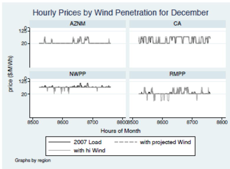
Figure 6. Energy market prices for December
