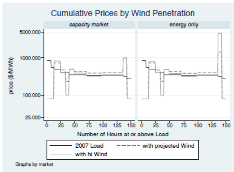
Figure 9. Highest 150 prices RMPP
