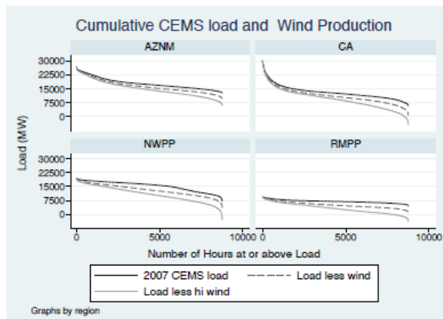
Figure 4. Annual distribution of CEMS load net of wind
