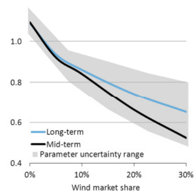
Figure 33. Parameter uncertainty. The shaded area indicates the upper and lower extremes of mid- and long-term runs.
