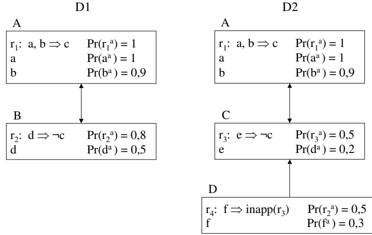
Figure 1: Dialogues generated from the mad cow example.
