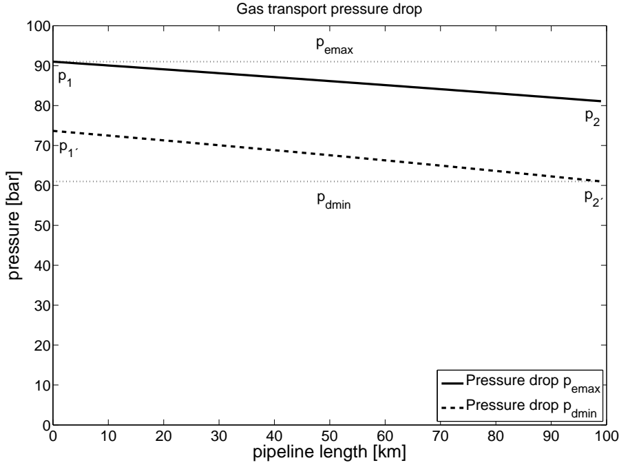
Figure 1: Line-pack flexibility: the area defined by p_1 p_2 p_2' p_1' represents the storage potential in the pipeline while simultaneously ensuring the transport corresponding to the pressure differential p_1^2 - p_2^2 at the lower boundary
