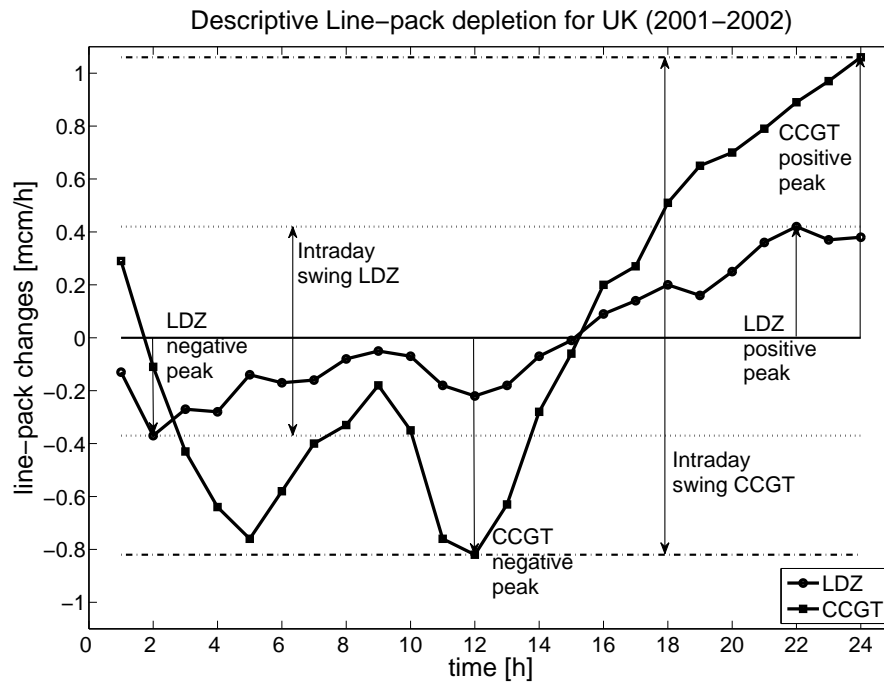
Figure 4: Description of the maximum hourly line-pack depletion for local distribution zones (LDZ) and combined cycle gas turbines (CCGT) in UK (2001-2002) (author elaboration, data from Lapuerta, 2003 and OFGEM, 2003)
