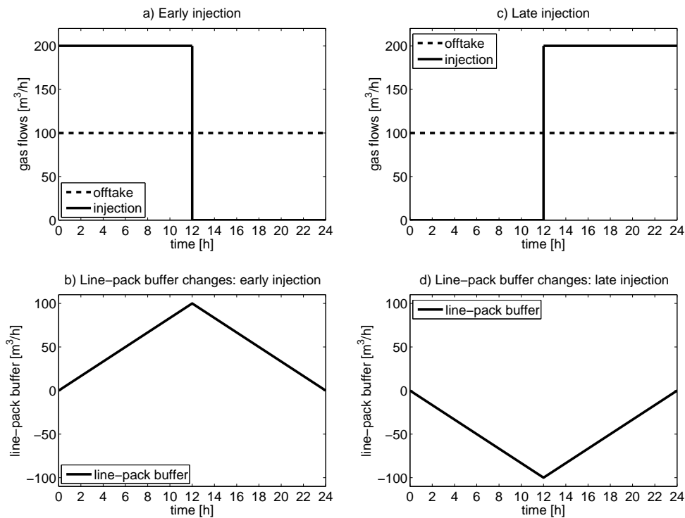
Figure 2: Accommodation of different gas injection and offtake time pattern: (a) early injection ( \text{m}^3/\text{h} ), (b) line-pack buffer creation ( \text{m}^3/\text{h} ), (c) late injection ( \text{m}^3/\text{h} ), (d) line-pack buffer extraction ( \text{m}^3/\text{h} )
