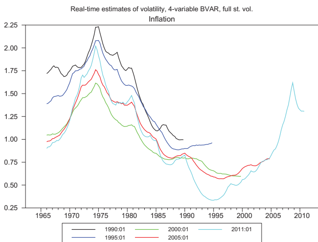
Figure 6: Volatility estimates from 4-variable BVAR with independent stochastic volatilities, real-time data
