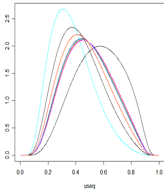
Posteriors for 10 respondents, response pattern 33323
