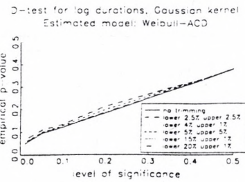
Figure 3: Size and power against exponential alternative, Weibull ACD
