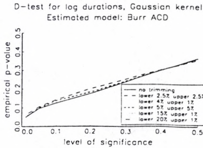
Figure 1: Empirical size, Burr ACD
