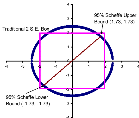
Panel 2 – 95% Confidence Circle for Orthogonalized Forecast Path
